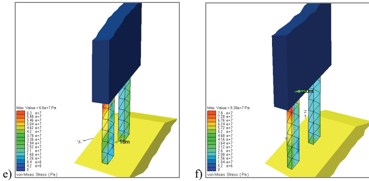
Fig. 6. a)–f) Security pillars 10 × 10 m loaded with weight in the ceiling part
