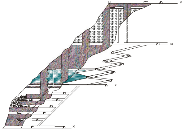
Fig. 2. The exploitation method in “Trepça” mine
