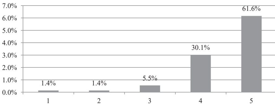
Fig. 3. Distribution of grades concerning the statement “the ISO 9000 series of standards contribute to promoting (spreading) the quality management in practice”
