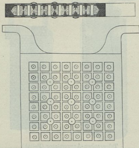
Kapsel-Elektrode (Morian &amp; Co., Neumühl).
