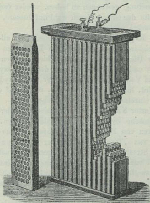
Kabath-Accumulator.
