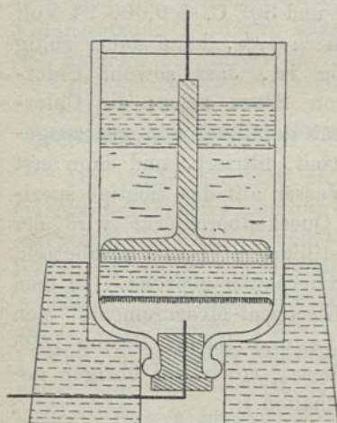
Normalelement (Helmholtz-Carhart).
