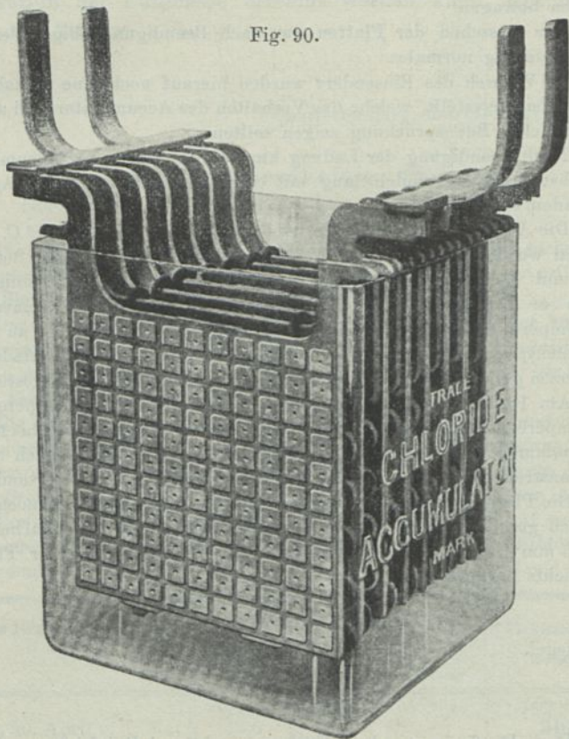
Chloride-Accumulator.
