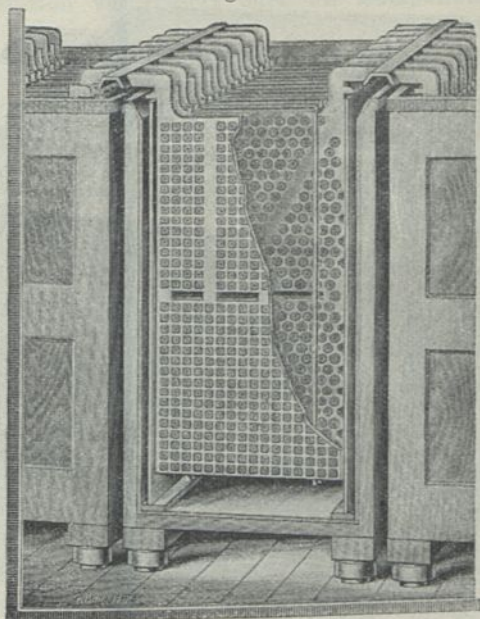
Accumulator der Chloride-Accumulator-Co.
