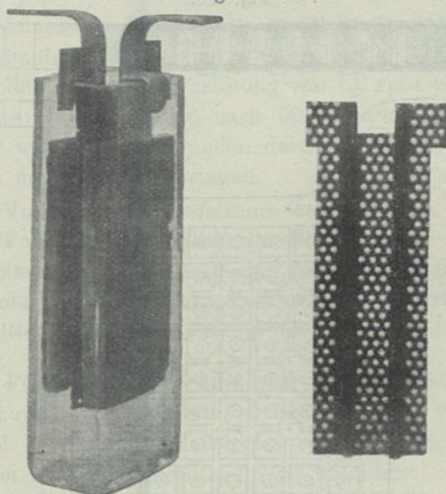
Telegraphen-Accumulator (Pollak).
