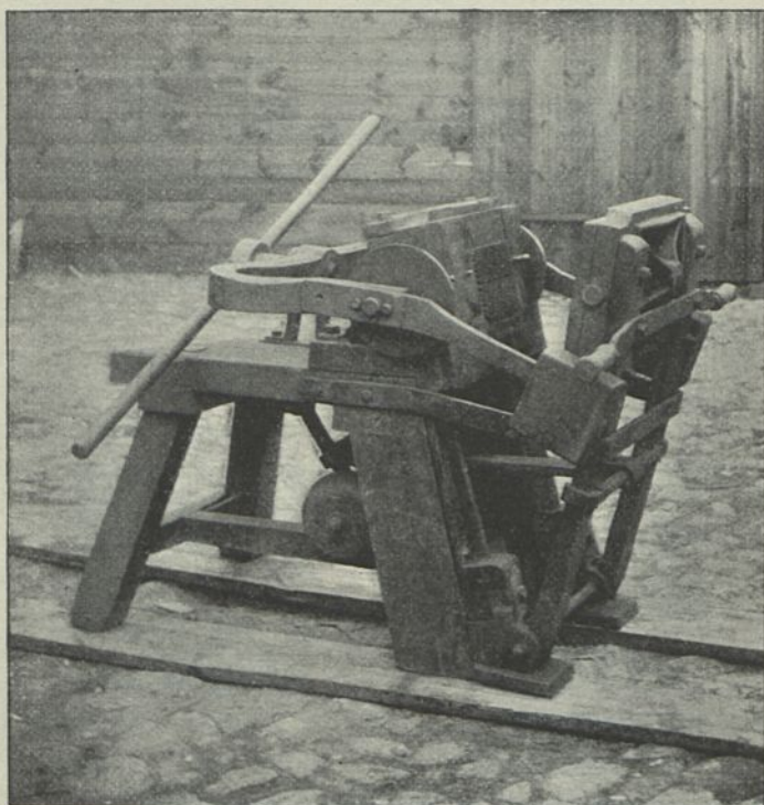
Correns-Gussform, offen.
