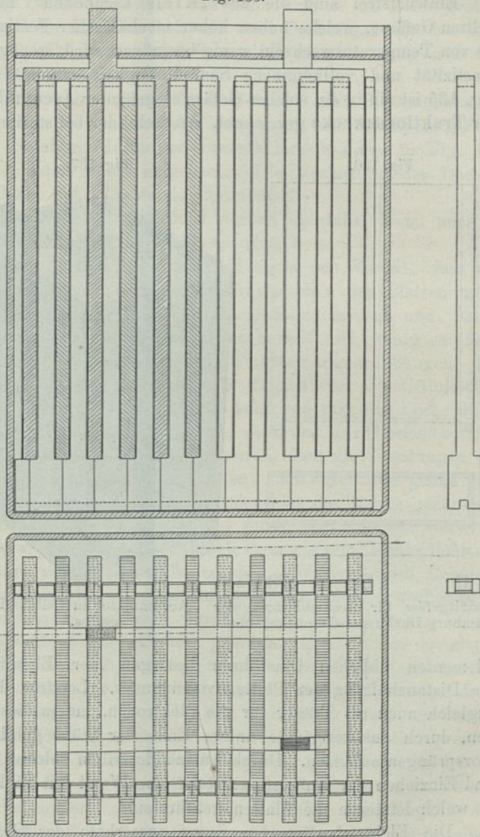
Element (transportabel) der American-Battery-Co.
