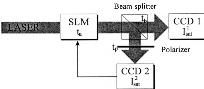
Fig. 3. Optoelectronic thresholder and binarisation system based on a SLM and a CCD.
