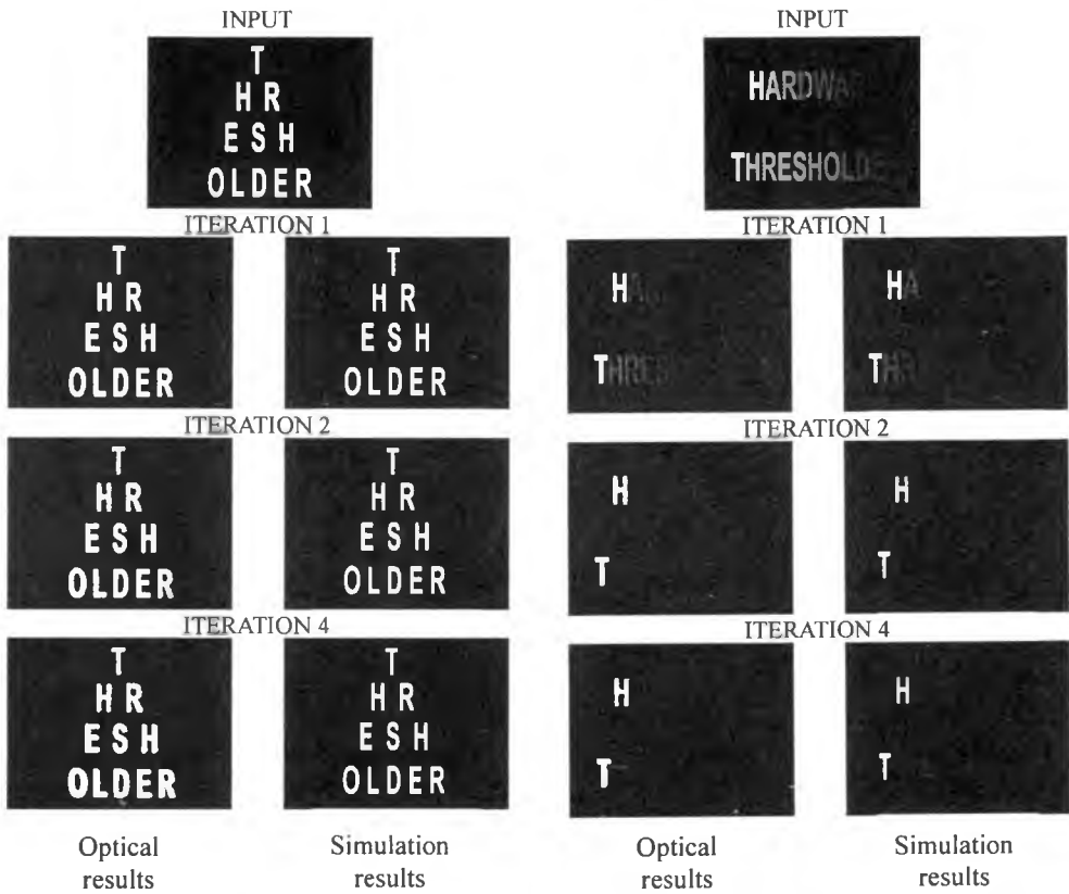
Fig. 6. Example of the work of the binarising setup for binary signal.
