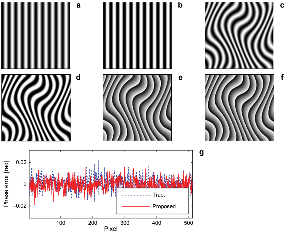
Fig. 7. Simulation results for the traditional three-step phase-shifting method ( a , c , e ) and the proposed third harmonic injection method ( b , d , f ). The reference fringe patterns of the two methods are shown in ( a ) and ( b ). ( c ) and ( d ) show the modulated patterns by the phase map shown in Fig. 6. The warped phase is shown in ( e ) and ( f ) and the cross-sections of the phase error are shown in ( g ).
