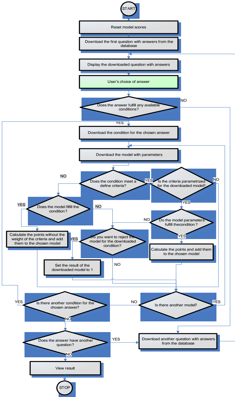
Fig. 3. Algorithm for selecting an SDLC model – a flowchart
