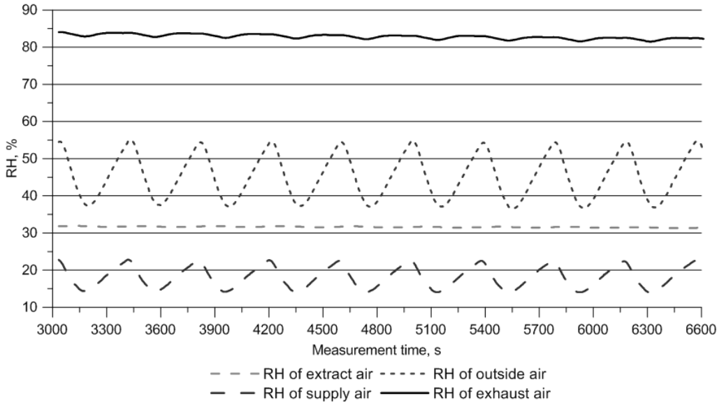
Fig. 3. Sequence of changes in relative humidity of the outside air for the outside air temperature of 5°C and 24°C – temperature of removed air
