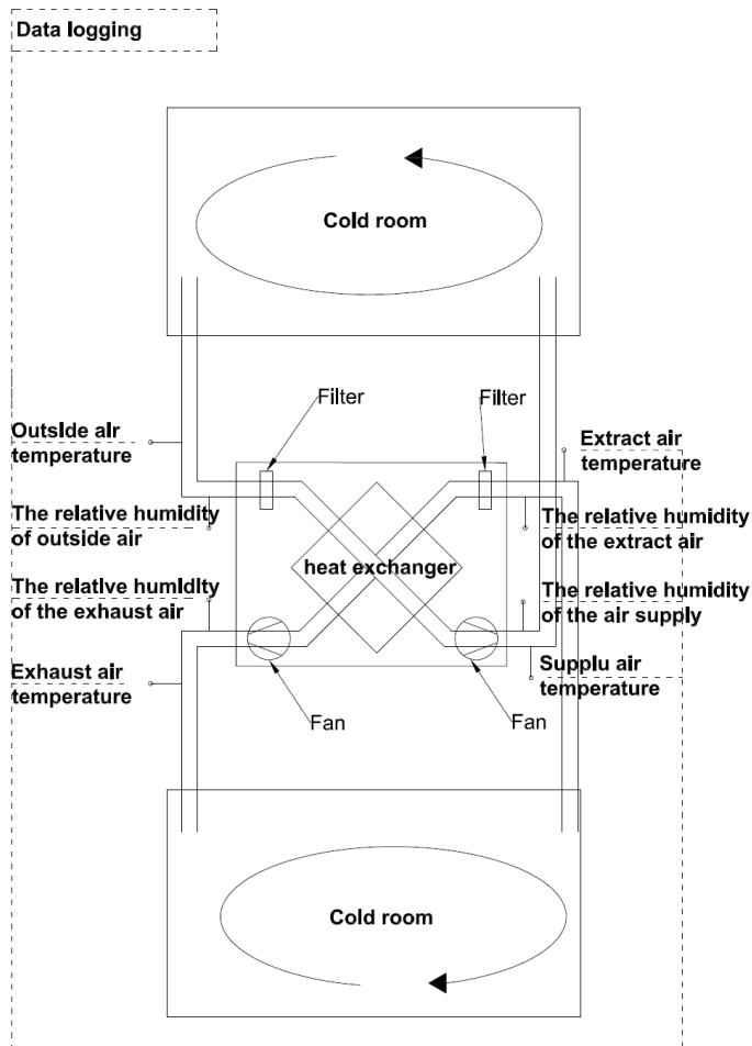
Fig. 1. The scheme of the testing-bench for heat exchangers and construction of the plate heat exchanger
