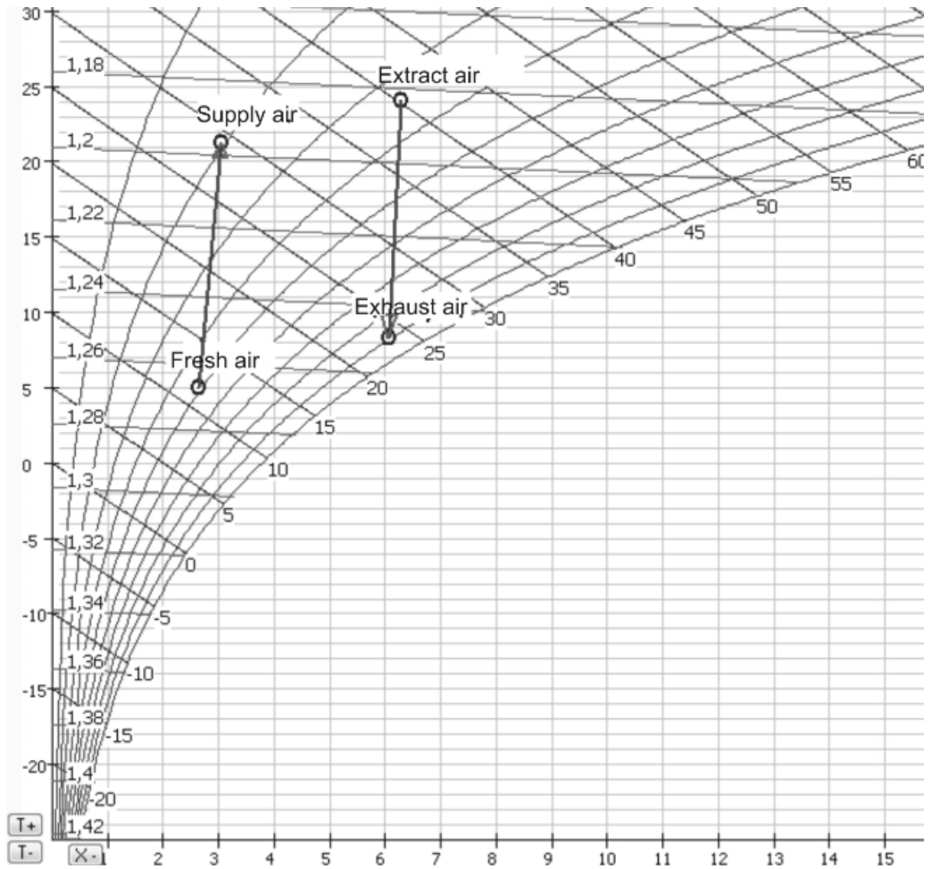
Fig. 5. Changes of air flowing through the heat exchanger for the outside air temperature of 5°C and 24°C – temperature of removed air
