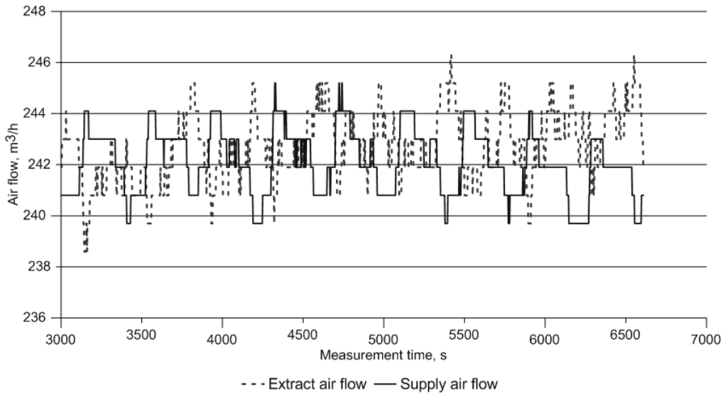
Fig. 4. Sequence of changes of air flow for exhaust and outside air for the outside air temperature of 5°C and 24°C – temperature of removed air
