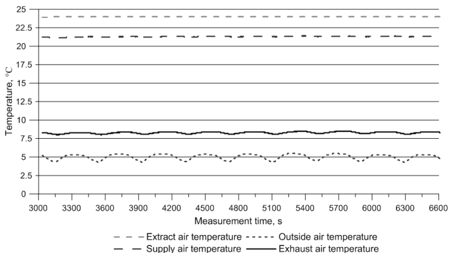
Fig. 2. Sequence of changes in temperature after stabilization system for the outside air temperature of 5°C and 24°C – temperature of removed air
