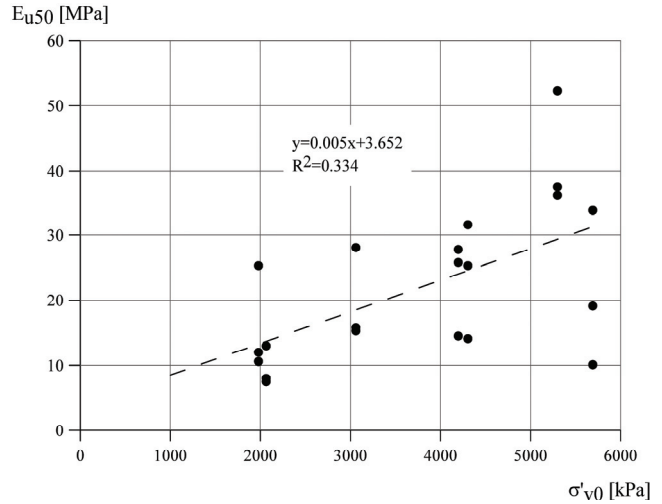
Fig. 3. The undrained modulus E_{u50} versus effective vertical stress in situ \sigma'_{v0}
