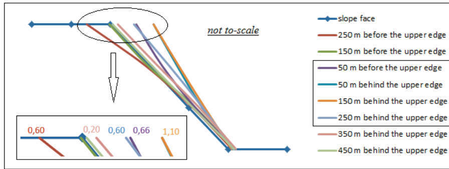
Fig. 12. Horizontal displacements of slope face at different positions of longwall panel (measured point is the center of the longwall panel)
