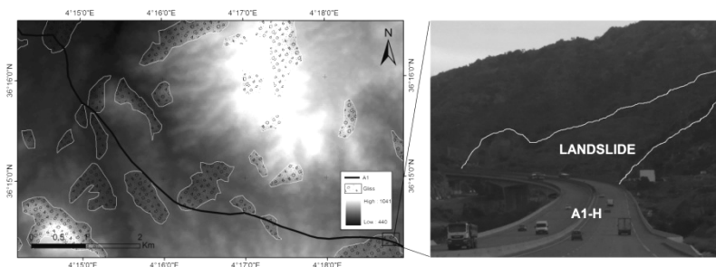
Fig. 1. Landslides inventory of the study area
