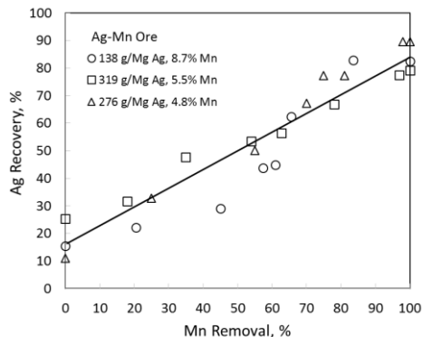
Fig. 6. Ag recovery in cyanide leaching as a function of manganese removal from Ag-Mn ore samples
