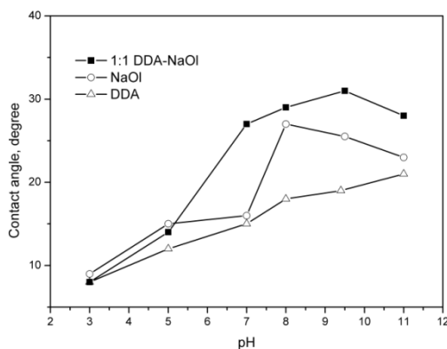
Fig. 1. Contact angles of FA with collectors as a function of pH (concentrations of DDA, NaOl and their mixtures all were 1 \cdot 10^{-4} mol/dm 3 )
