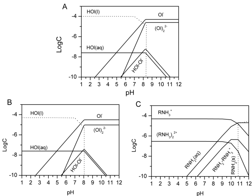
Fig. 2. Species distribution diagrams of oleate (A, 1 \cdot 10^{-4} \text{ mol/dm}^3 ; B, 5 \cdot 10^{-5} \text{ mol/dm}^3 ) and DDA (C, 5 \cdot 10^{-5} \text{ mol/dm}^3 ) as a function of pH
