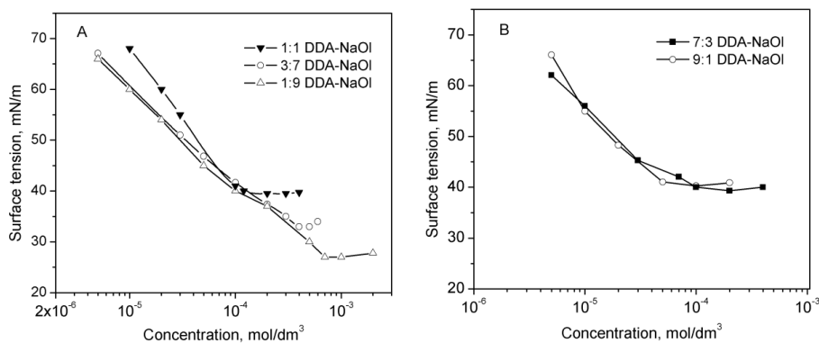
Fig. 3 Surface tension results of DDA-NaOl mixtures at pH 9.5
