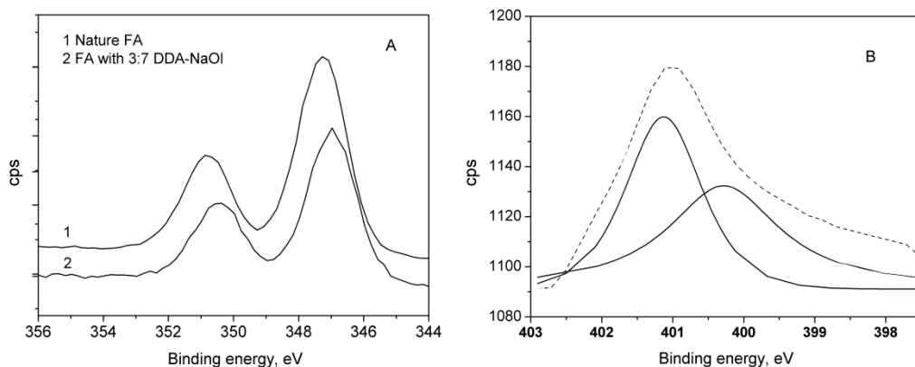
Fig. 6. XPS results of Ca2p peaks (A) and N1s peaks (B) of FA treated with the 3:7 DDA-NaOl mixture
