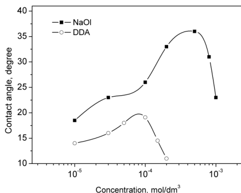
Fig. 4. Contact angles at FA surface depending on the NaOl and DDA concentrations at pH 9.5
