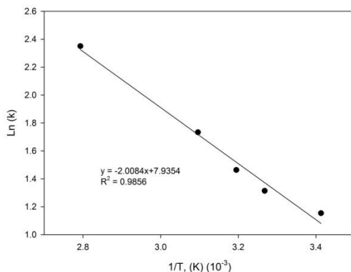
Fig. 13. The Arrhenius plot for dolomite dissolution at various temperatures
