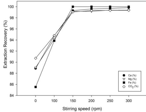
Fig. 8. Effect of stirring speed on sample dissolution recovery
