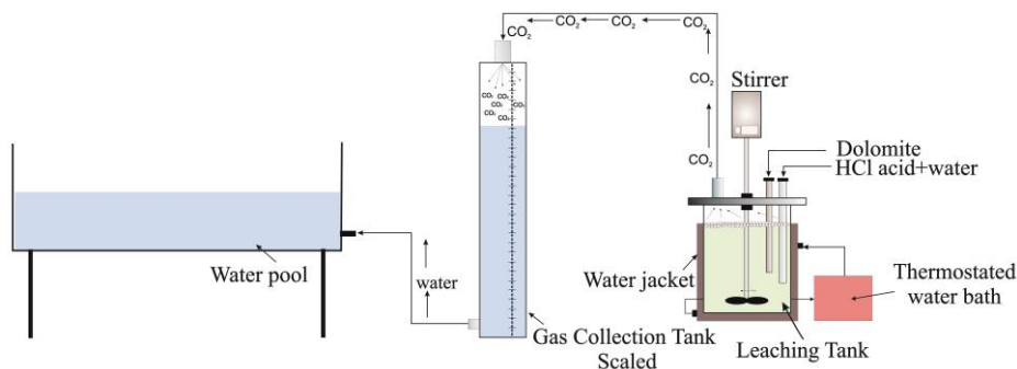
Fig. 2. Experimental set-up for dissolution of dolomite ore
