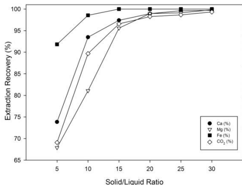
Fig. 6. Effect of solid/liquid ratio on sample dissolution recovery
