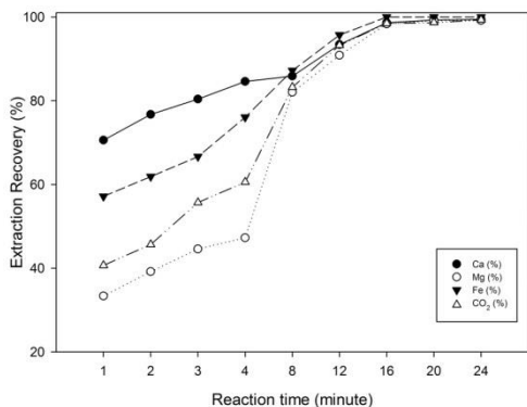
Fig. 7. Effect of reaction time on sample dissolution recovery
