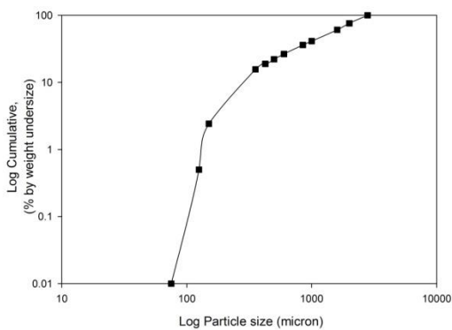
Fig. 4. Particle size distribution of the sample -2.80 mm in sized
