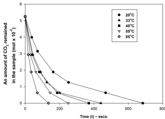
Fig. 10. CO 2 amount remained in sample after leaching experiments at various temperatures
