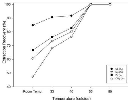
Fig. 10. Effect of temperature on sample dissolution
