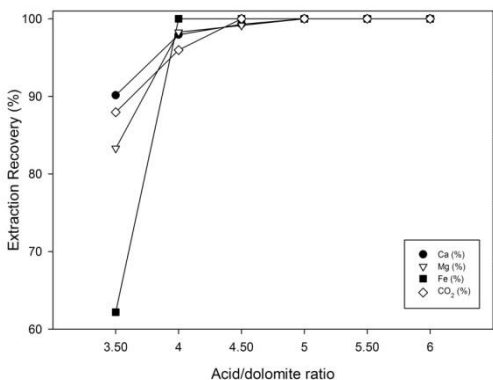
Fig. 5. Effects of acid/dolomite ratio on dissolution recovery of the sample
