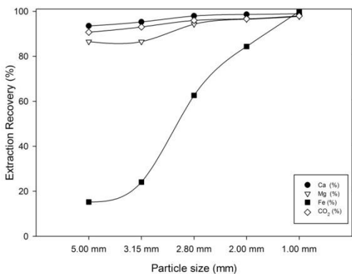
Fig. 3. The effects of particle size on dolomite dissolution
