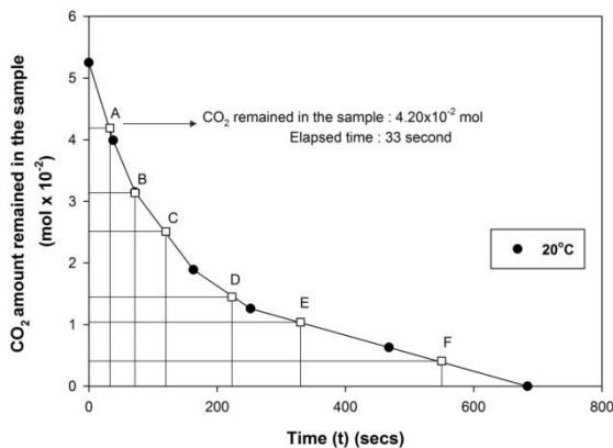
Fig. 11. Determination of CO 2 amount ( 0.8 \cdot C_{A0} ) from the curve
