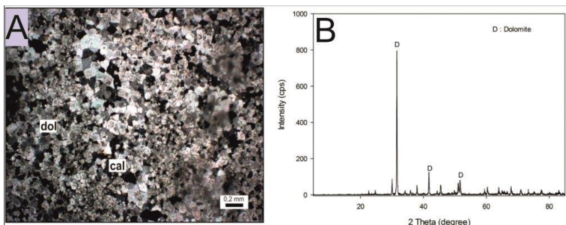
Fig. 1. Thin-section photograph (A) under microscope and XRD pattern (B) of the sample
