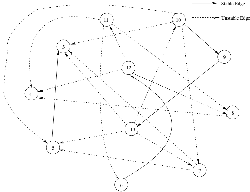
Figure 3. The induced subgraph of dependency graph of the sequence diagram in Figure 2 on the node set {3, 4, 5, 6, 7, 8, 9, 10, 11, 12, 13}
