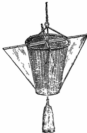
FIG. 1.—CURRENT DRAG
