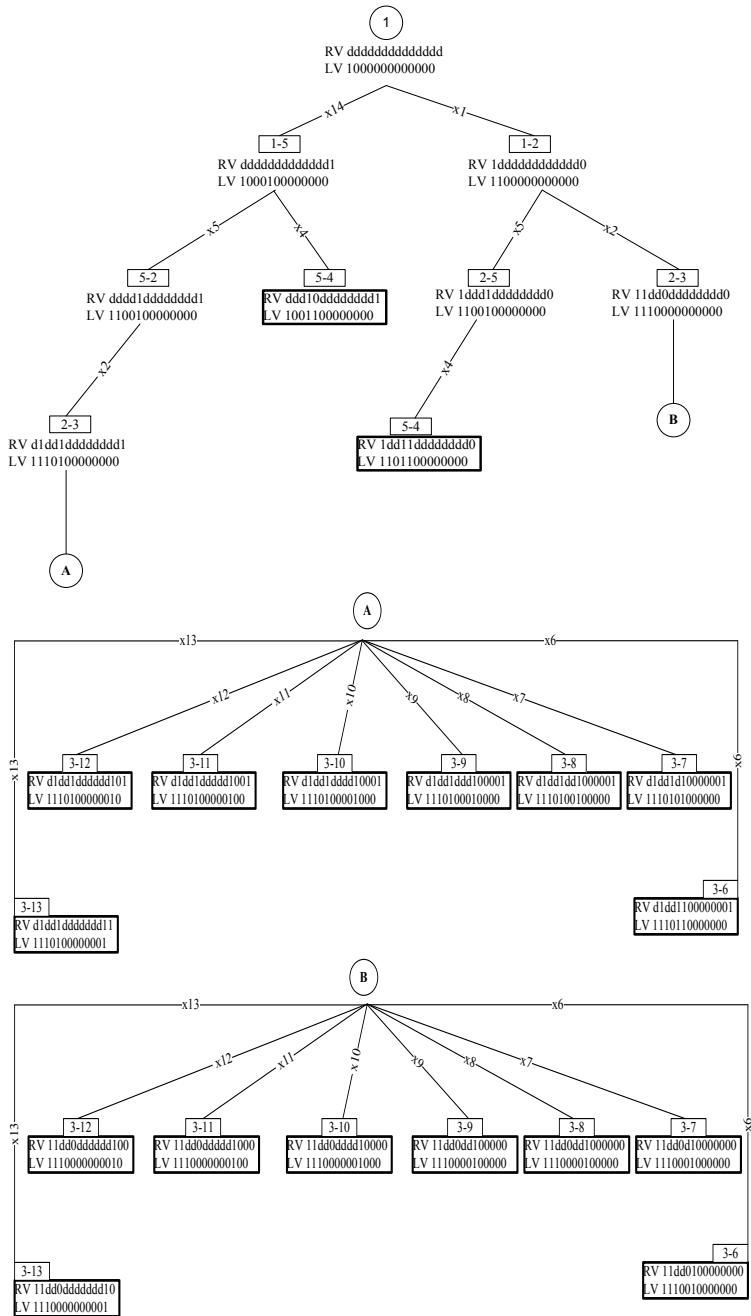
Figure 8. A complete tree for evaluating DSR in IIS
