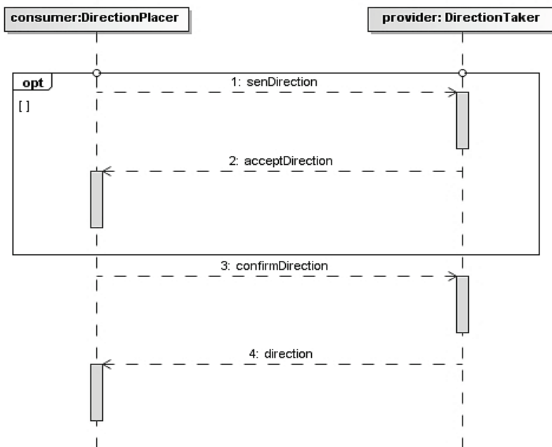
Figure 5. Specification of the Direction service choreography (behavior)
