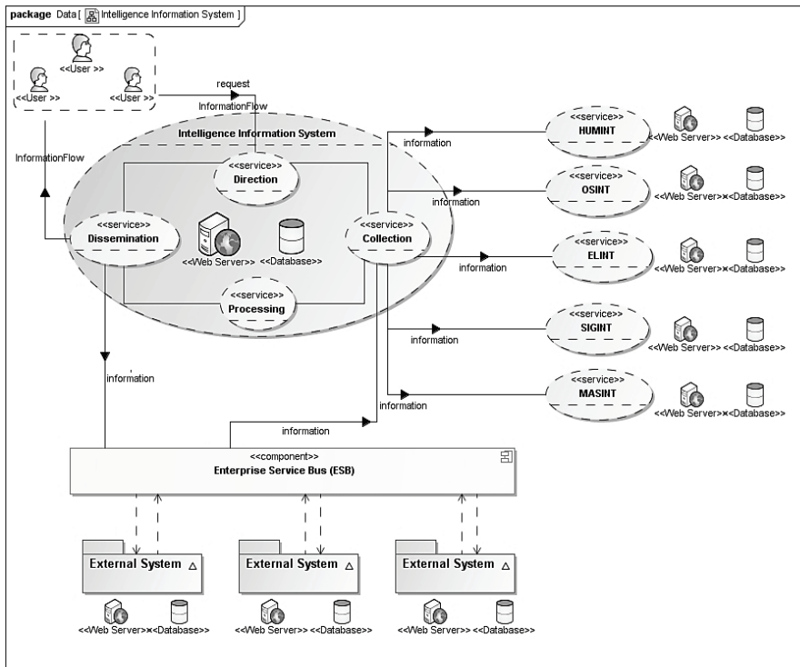
Figure 6. The dataflow in the Intelligence Information System – based on SOA
