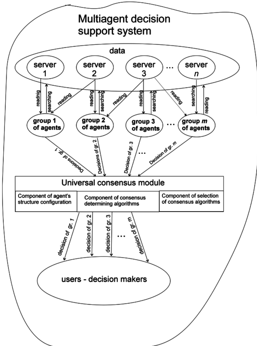
Figure 1. Diagram of multi-agent decision support system including consensus module
