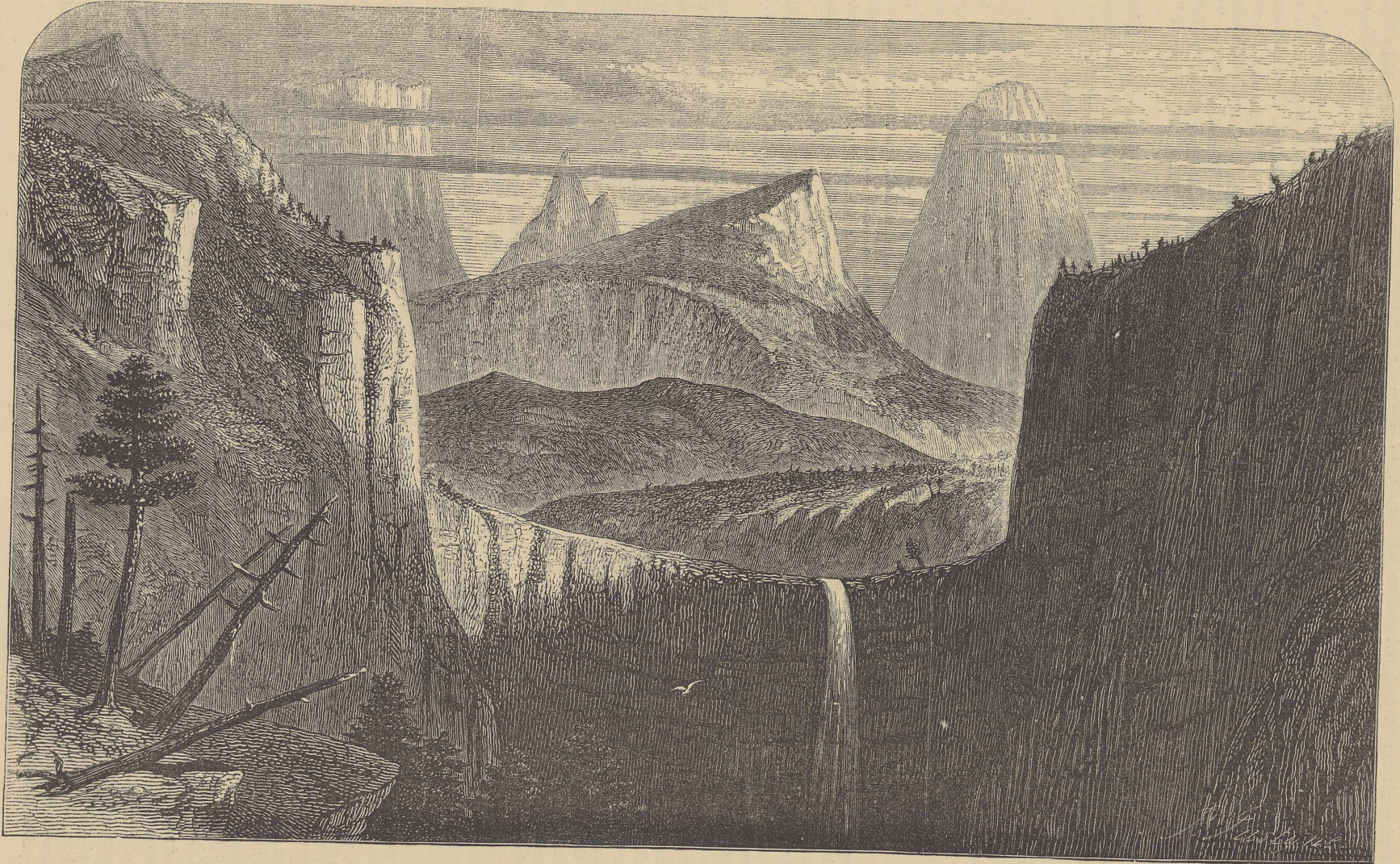
VIEW OF PART OF THE MERCED CANON WITH THE VERNAL FALL, YOSEMITE VALLEY, CALIFORNIA (From Report on Geological Survey of California by C. J. D. Whitney, State-Geologist)
