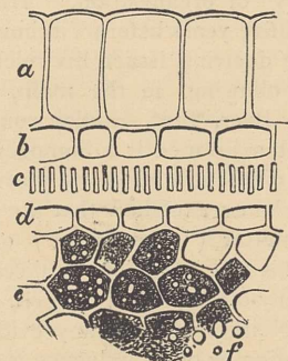
Fig. 2.—Section of a flax-seed, highly magnified, exhibiting a cells containing mucilage, e cells containing caseine and drops of oil f .
