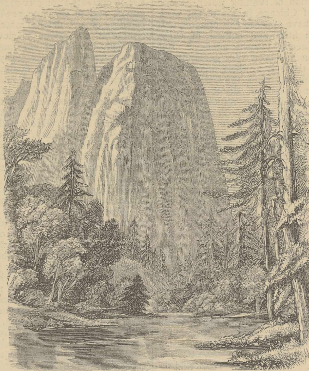
HEAD OF MERCED AND TUOLUMNE RIVERS (See Geology of the Sierra Nevada in Whitney's Geological Survey of California, pp. 415-419)
