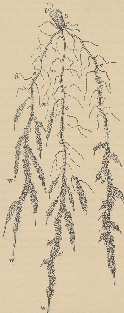
Fig. 5.—Young wheat plant with earth adhering to roots at e , while the root tips w , and the other parts of the primary roots e , and of the secondary roots n are bare. S is the seed and b the blade.
