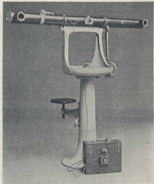
FIG. 3.—Barr and Stroud range-finder on fortress mounting.
