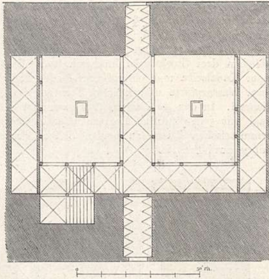
Abb. 198. Pal. Pizzardi zu Bologna. (L.)
