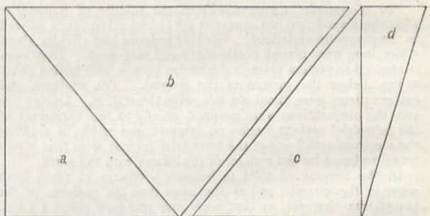
a, calc-spar; b, calc-spar; c, crown glass; d, dense flint glass.
