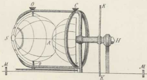
Fig. 2 Front Elevation
