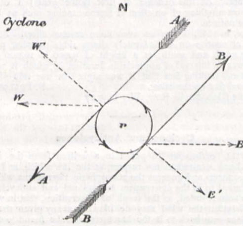
CYCLONE.—AA, a north-east wind; BB, a south-west wind; w, westerly drift of AA due to difference of absolute velocities of earth's motion at different latitudes; w', effective part of w, in producing rarefaction at r; E, effective part of E as above. Result, rarefaction in centre of cyclone.
