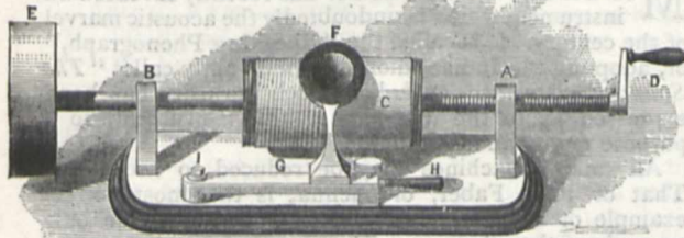
FIG. 1.—Edison's Talking-Phonograph.
