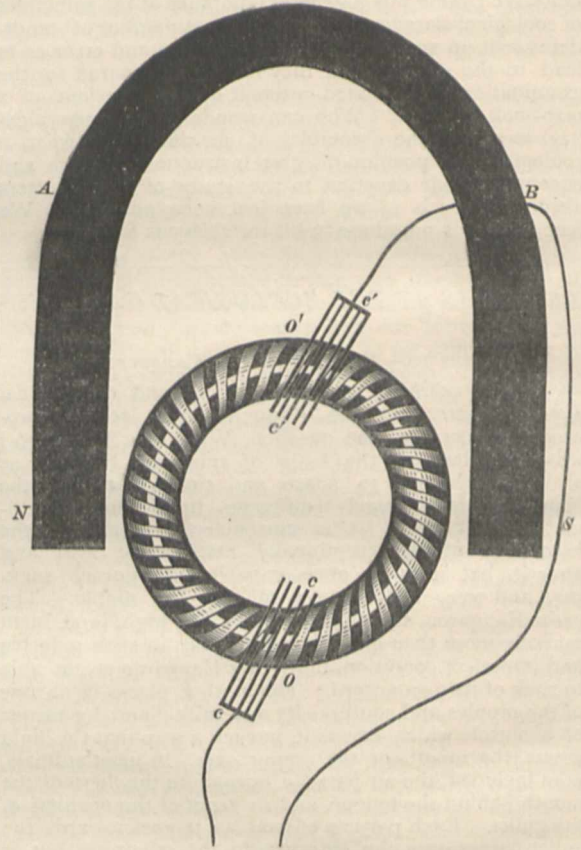
FIG. 4.—Ring Armature.
