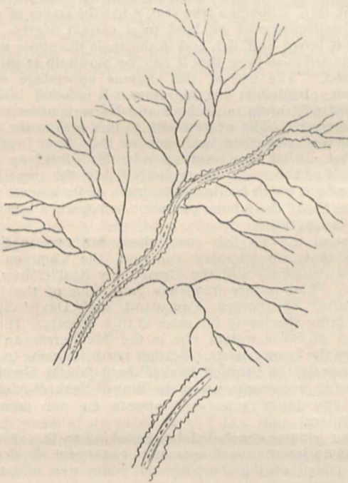
FIG. 1.—Breath Figure of Electric Discharge (also called Roric Figure , from Ros-ros is , "dew.")
