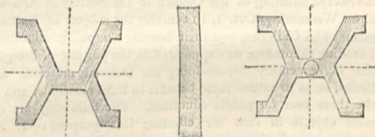
FIG. 14.—Form of New Standard Metres.
