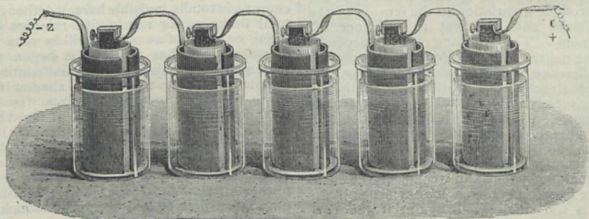
FIG. 12.—Pile formed by five Bunsen's elements.
