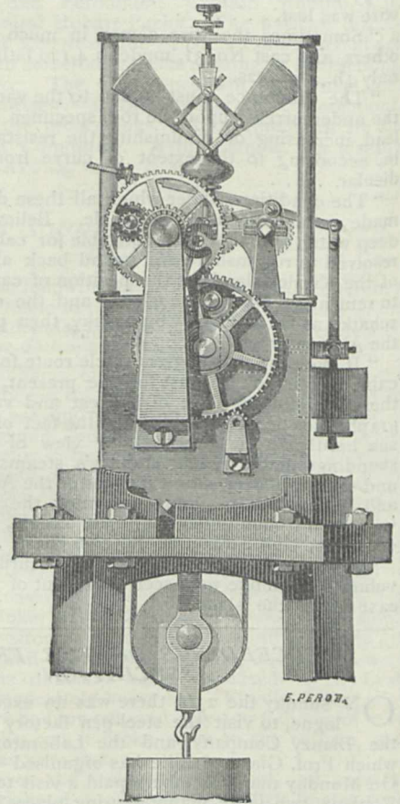
FIG. 2.—Clockwork movement, with isochronous regulator
