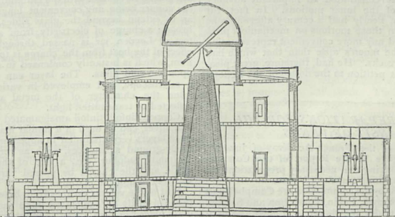
FIG. 5.—Section of Main building—United States Naval Observatory, 1844.
