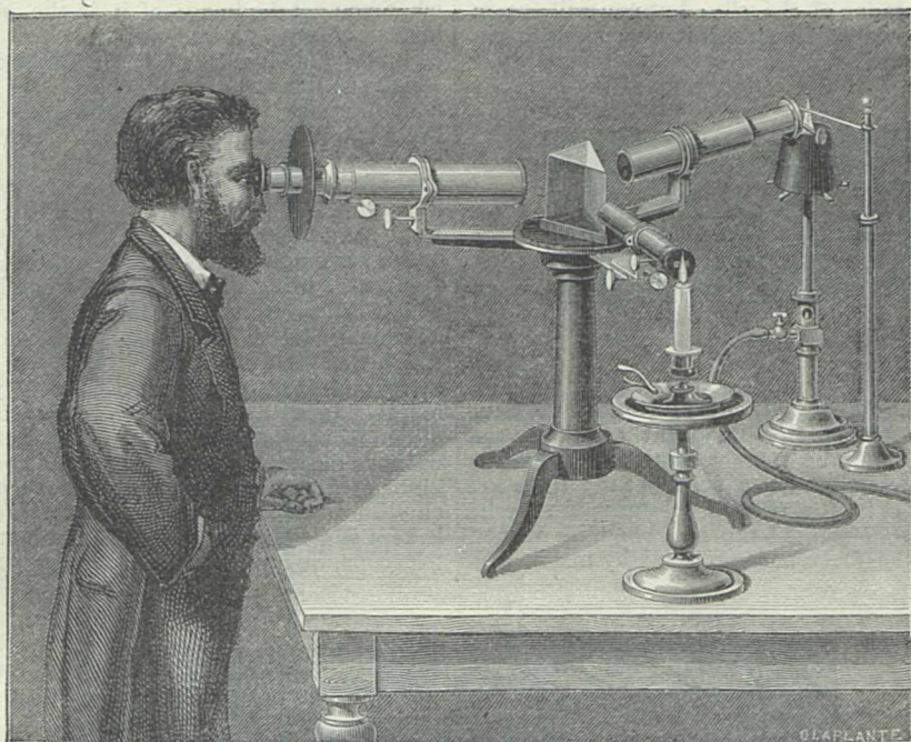
FIG. 15.—Spectroscope with reflected scale.
