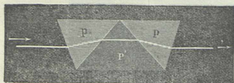
FIG. 17.—Direct-vision prism with three prisms.
