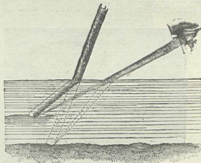
FIG. 4.—Explanation of the bent stick.
