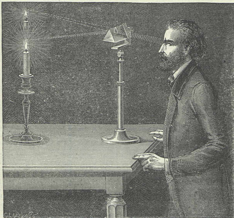
FIG. 8.—Images of objects seen through pri s ms.
