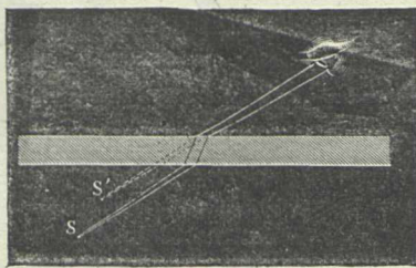
FIG. 6.—Light passing through plate of glass.
