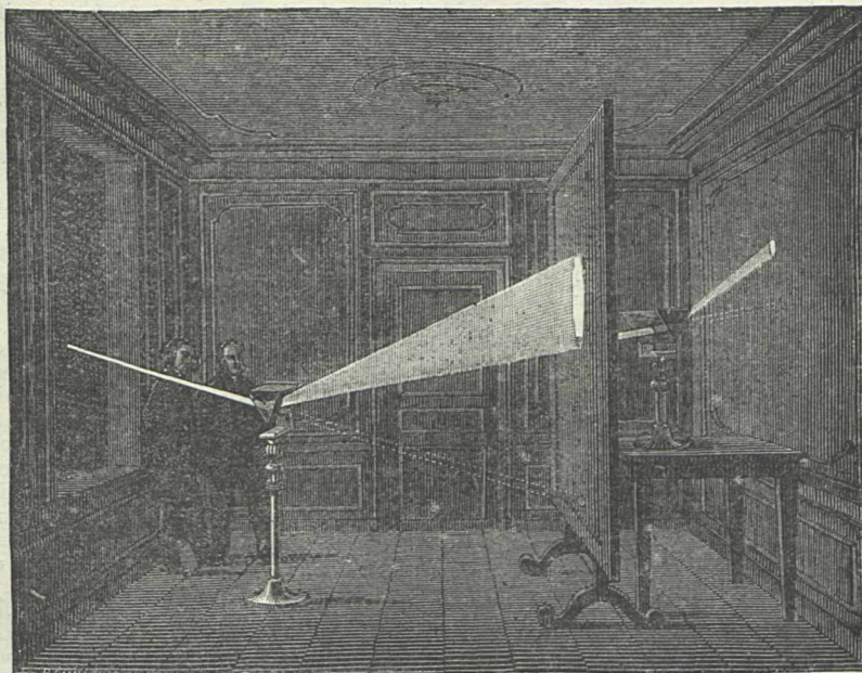
FIG. 9.—Decomposition of light by the prism. Unequal refrangibility of the colours of the spectrum
