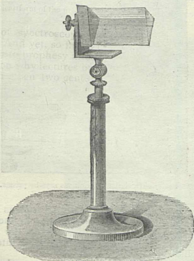
FIG. 2.—Prism mounted on a stand.
