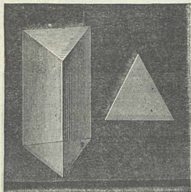
FIG. 1.—Geometrical-form of the prism.
