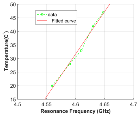
Fig. 5. Different temperatures of water versus resonance frequency.
