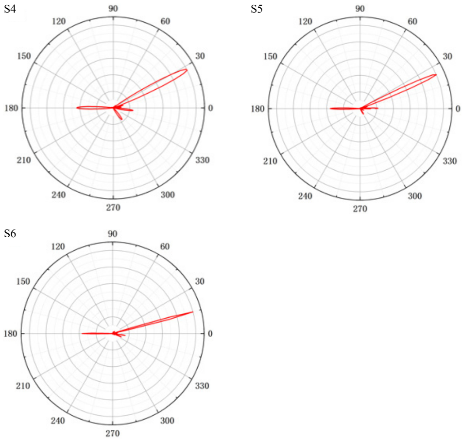
Fig. 18. Polar coordinate diagram of S4, S5, and S6.
