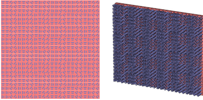
Fig. 33. Schematic and layout diagram of mixed coding sequence.
