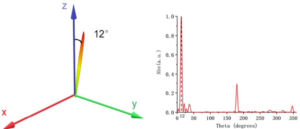
Fig. 22. 3D scattering angle of non-basic sequence S8.
