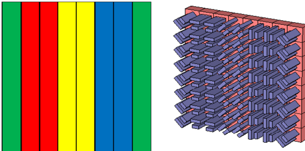
Fig. 19. Arrangement of non-basic sequence S7 .
