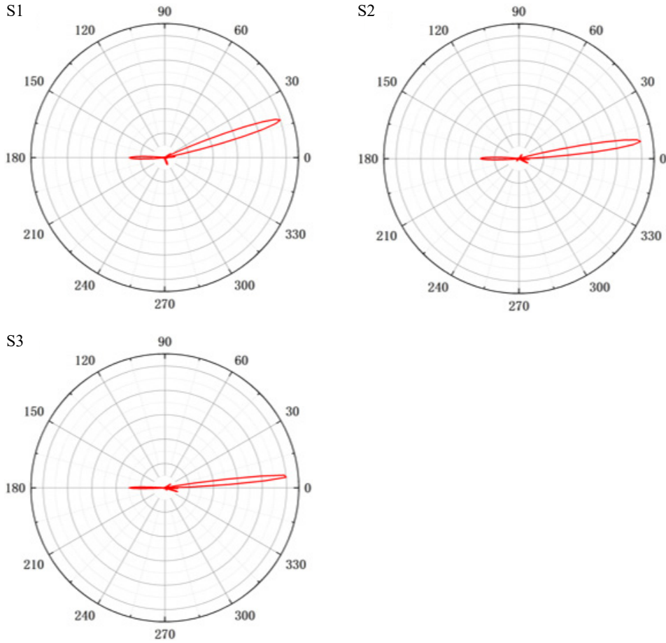
Fig. 11. Polar coordinate scattering of S1, S2, S3.
