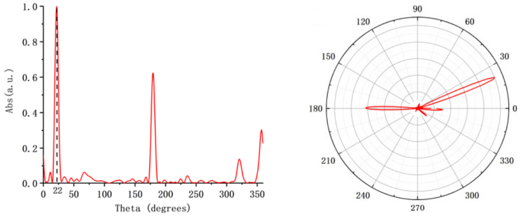
Fig. 38. The scattering results of 700 THz LCP incident on S4.
