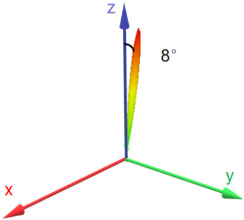
Fig. 9. Scattering angle of the basic sequence S2.
