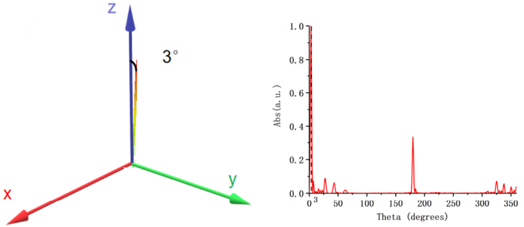
Fig. 24. 3D scattering angle of non-basic sequence S9.
