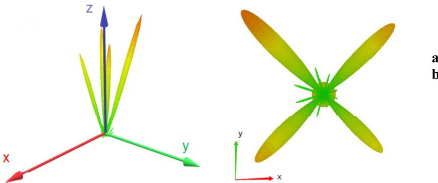
Fig. 32. Scattering of checkerboard coded metasurface, (a) stereo view, (b) top view.
