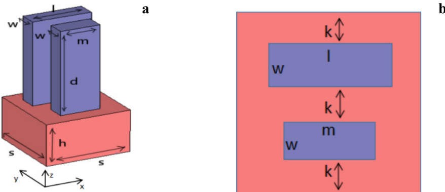
Fig. 2. Schematic diagram of metasurface unit structure.
