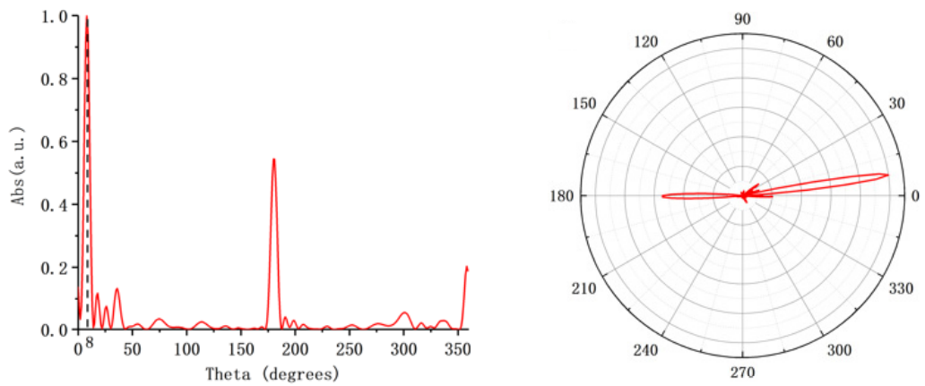
Fig. 40. The scattering results of 700 THz LCP incident on S7.
