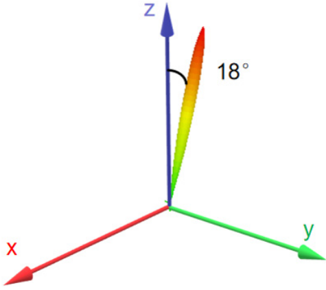
Fig. 8. Scattering angle of the basic sequence S1.
