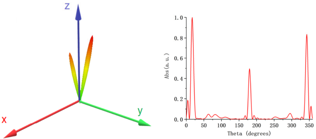
Fig. 28. Scattering angle of S10.
