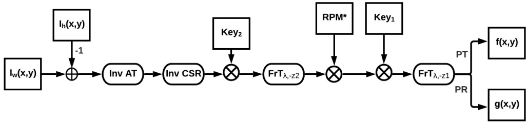
Fig. 2. Decompression and decryption process.
