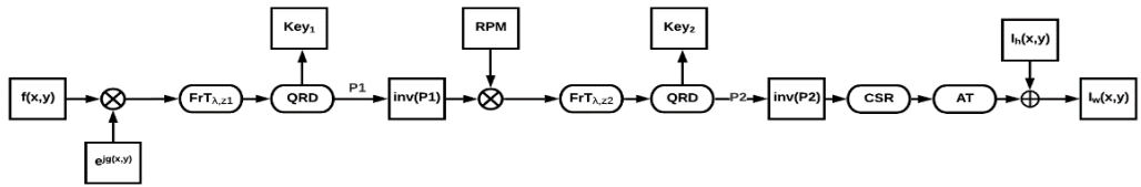
Fig. 1. Flowchart showing encryption, compression, and watermarking process.
