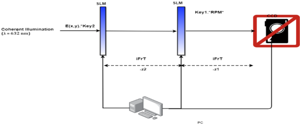
Fig. 3. Optoelectronic setup of the decryption process.
