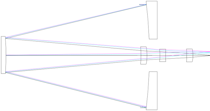
Fig. 4. Objective lens.
