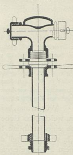
Standröhre. \frac{1}{10} w. Gr.
