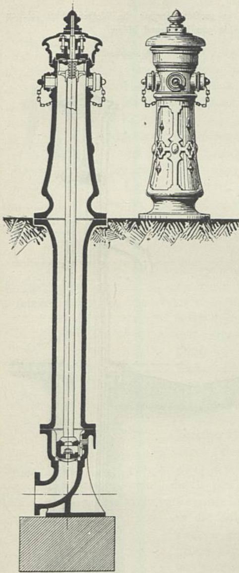
Ueberflur-Hydrant. — \frac{1}{25} w. Gr.
