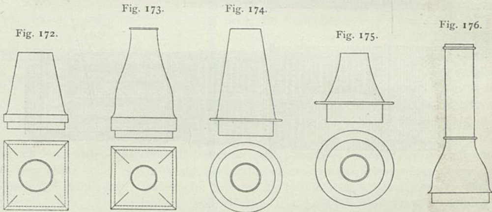
Schornsteinauffätze. — \frac{1}{10} w. Gr.
