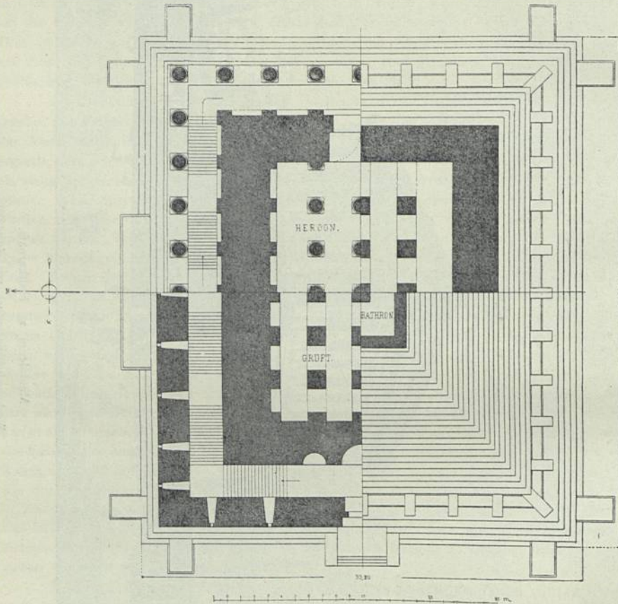
Mausoleum zu Halikarnafs.
