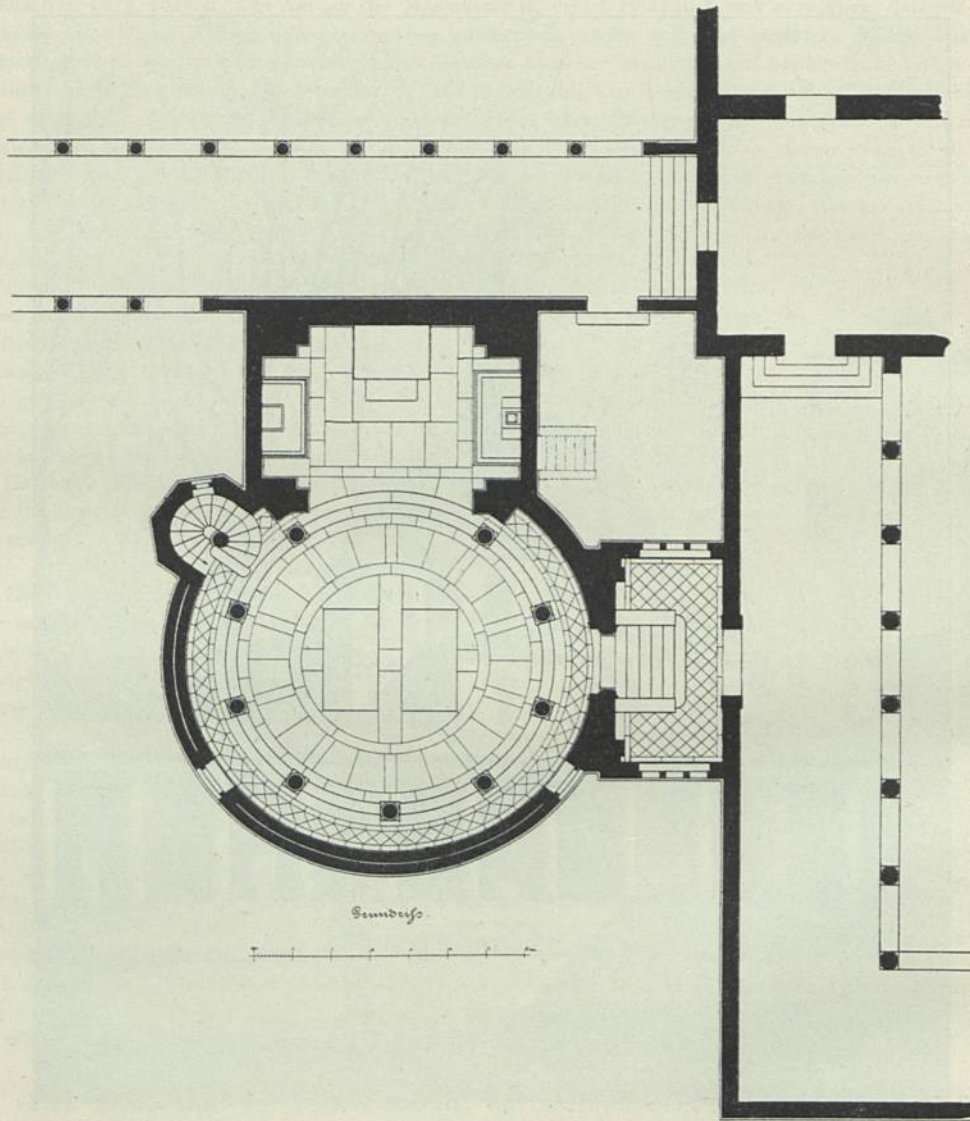
Kaiser Friedrich III. Mausoleum zu Potsdam.
