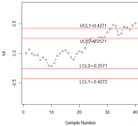
Fig. 1. Simulated control chart for the proposed procedure using RG sampling
