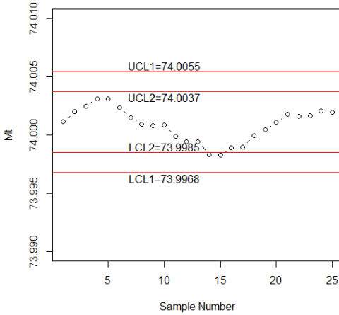
Fig. 5. Control chart for real data using RG sampling
