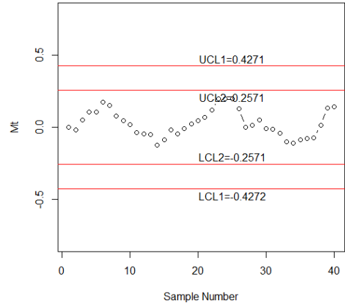
Fig. 2. Simulated control chart for the existing process using RG sampling
