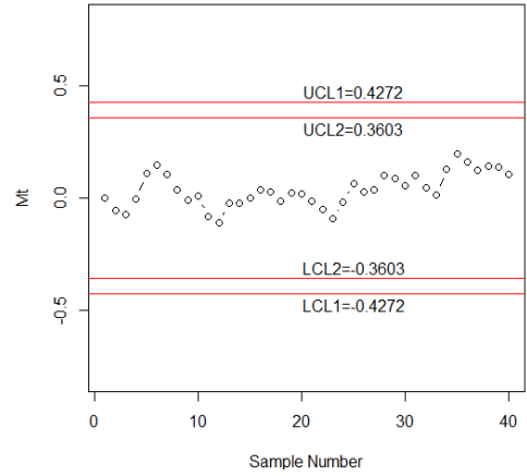
Fig. 4. Simulated control chart for the existing procedure using MDS sampling
