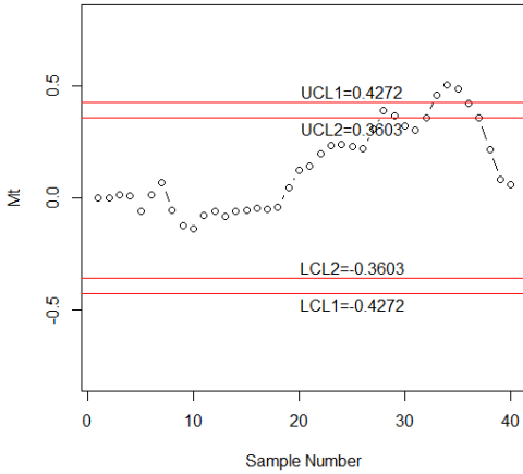
Fig. 3. Simulated control chart for the proposed procedure using MDS sampling
