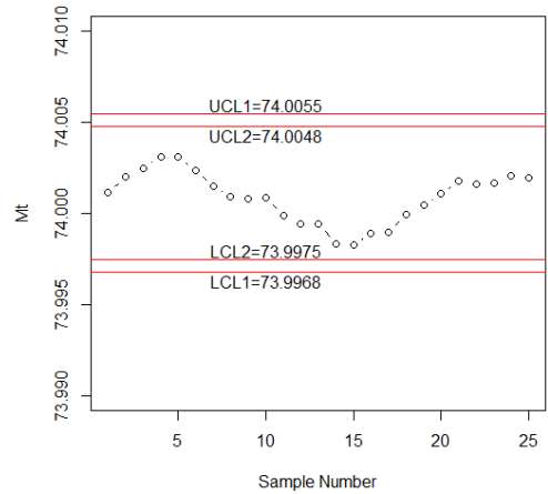
Fig. 6. Control chart for real data using MDS sampling
