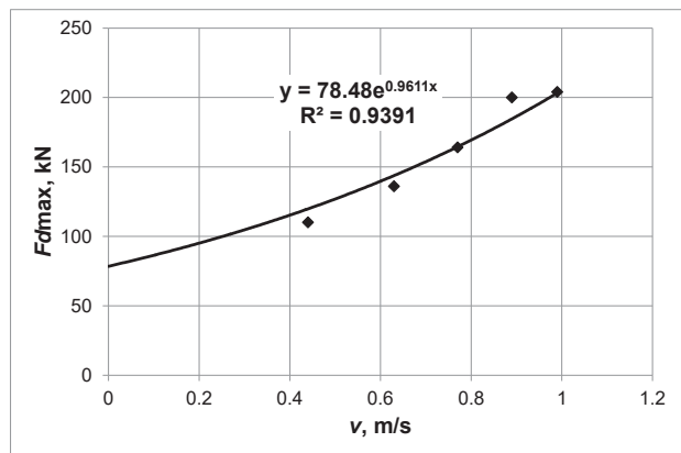
Figure 10: Relation of the maximum force as a function of impact velocity.
