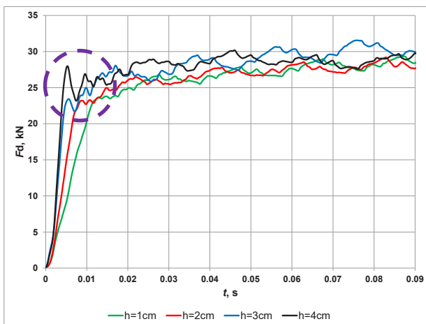
Figure 18: Courses of load F_d as a function of time t under dynamic bending loading of the bolt rods.
