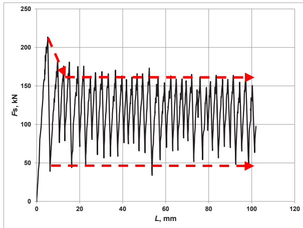
Figure 20: Course of load as a function of joint displacement under static load (maximum loading force F_{smax} = 213 kN).
