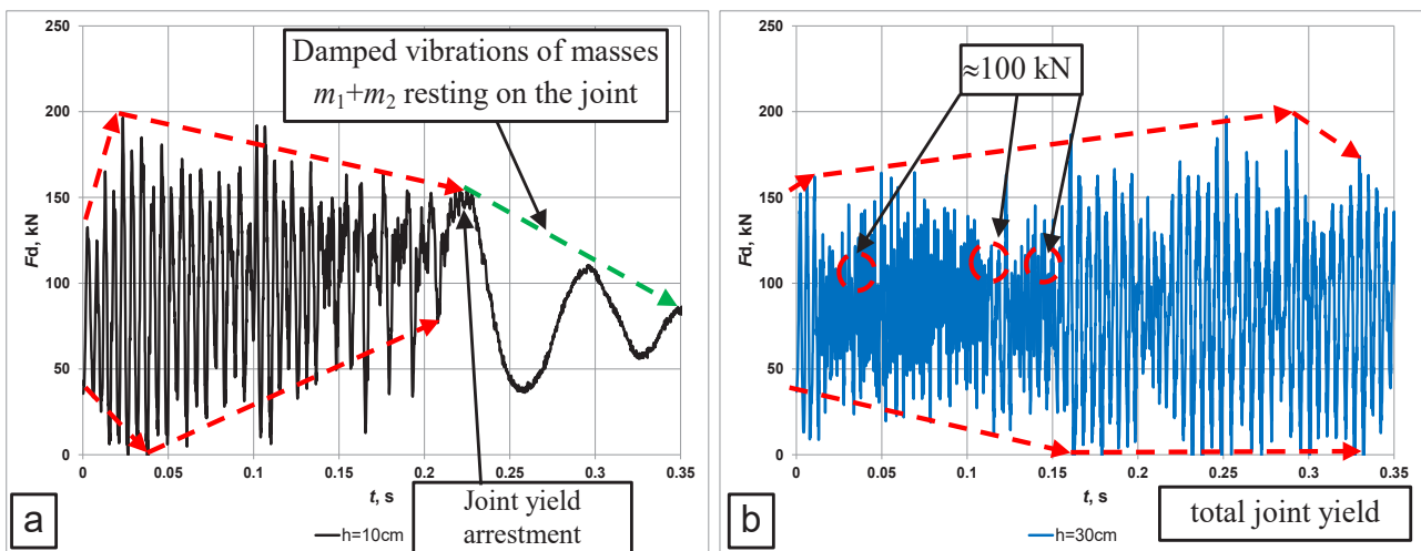
Figure 21: Course of load F_d as a function of time t under dynamic load of the joint at heights: h = 10 cm (a) and h = 30 cm (b).
