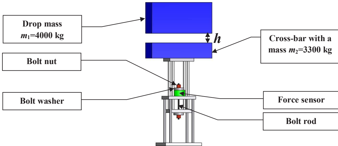
Figure 8: Test facility diagram.
