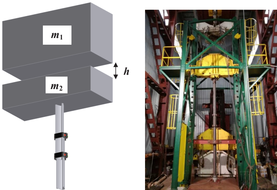
Figure 19: Diagram (left) and view (right) of the facility for sliding joint tests under dynamic load.
