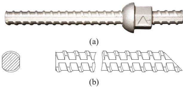
Figure 4: Bolt rod and nut: (a) – view of the rod with the nut; (b) – drawing of the rod with a trapezoidal thread and sectional view.
