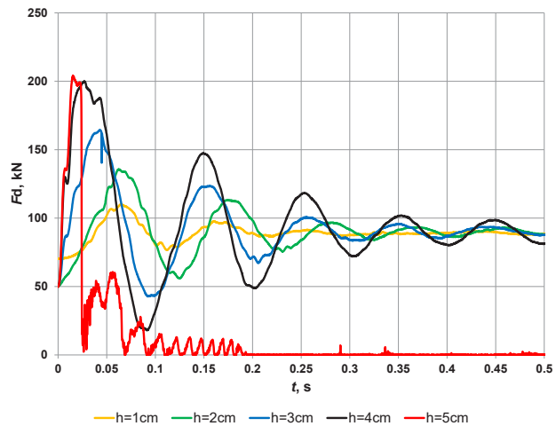
Figure 9: Courses of load as a function of time under dynamic tensile loading of the bolt rods.
