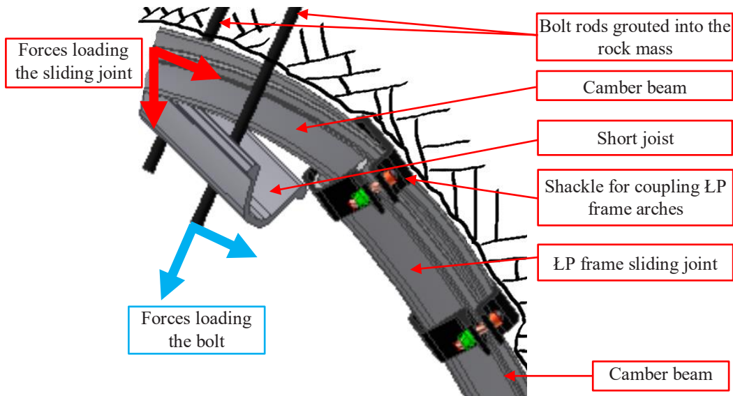
Figure 3: Loading diagram of the ŁP yielding support frame joint and bolts.
