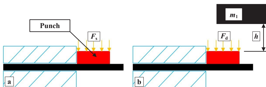
Figure 11: Diagram of the test stand for bolt rod shear tests under: (a) – static load; (b) – dynamic load.
