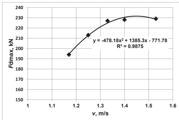
Figure 14: Relation of the maximum shearing force and impact velocity.
