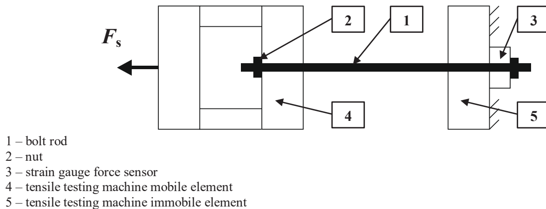
Figure 6: Test stand diagram for bolt tests under static load.
