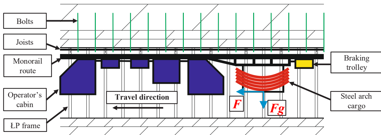
Figure 2: Mine working diagram with transportation via suspended monorail.
