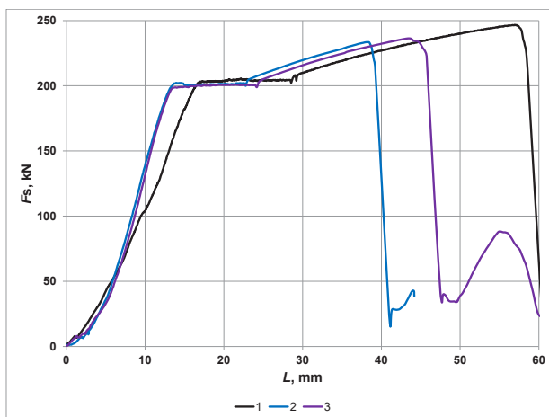
Figure 7: Courses of load as a function of elongation under static load.
