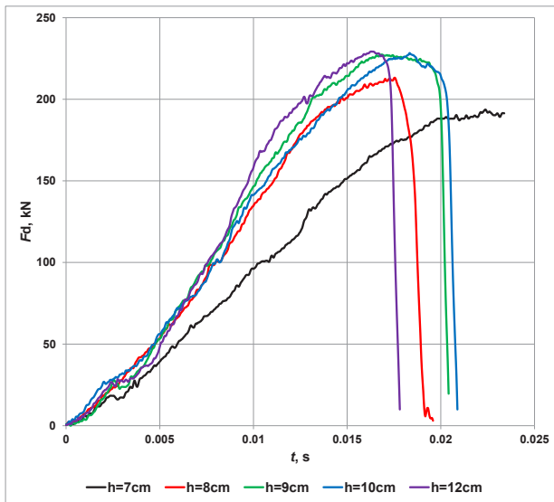
Figure 13: Relations of load as a function of time under dynamic shear loading of the bolt rods.
