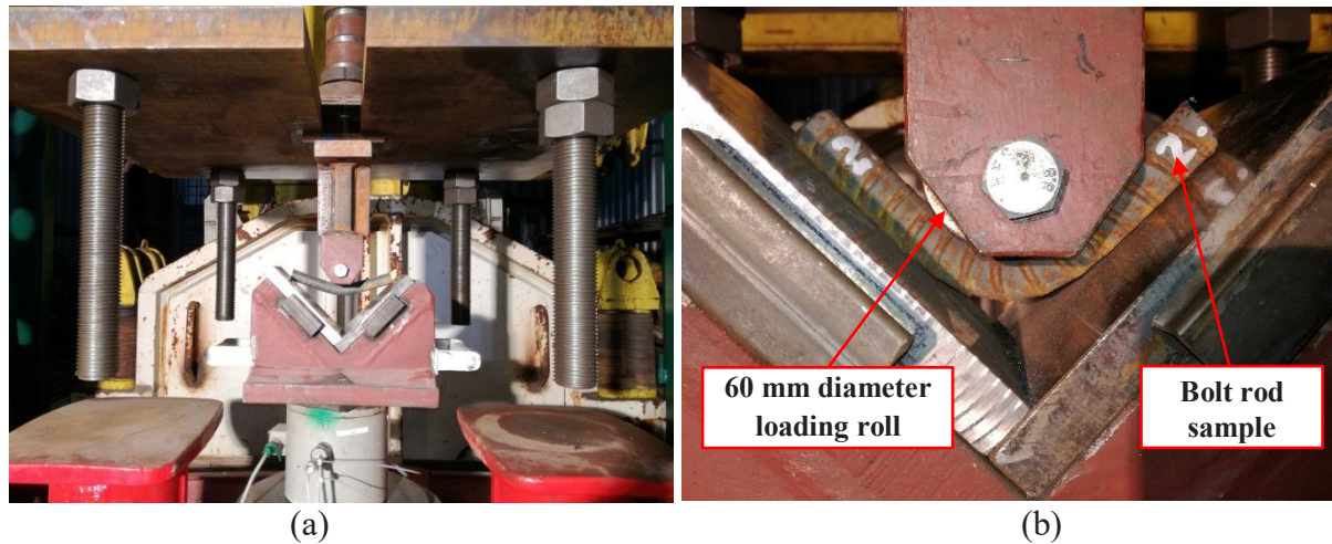
Figure 16: Test stand for bending strength tests under dynamic load: (a) – rod bending by an angle smaller than 90^\circ ; (b) – rod bending by 90^\circ .
