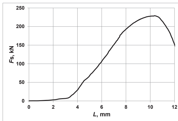
Figure 12: Relation of load as a function of bolt rod displacement during its shearing (maximum shearing force F_{smax} = 229 kN).
