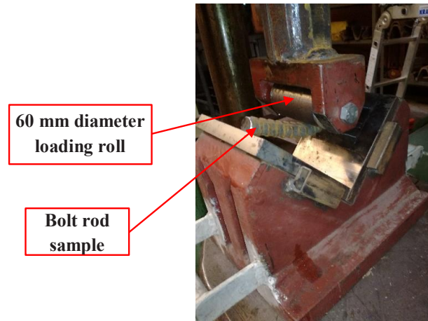
Figure 15: Test stand for bolt rod bending strength tests under static load.
