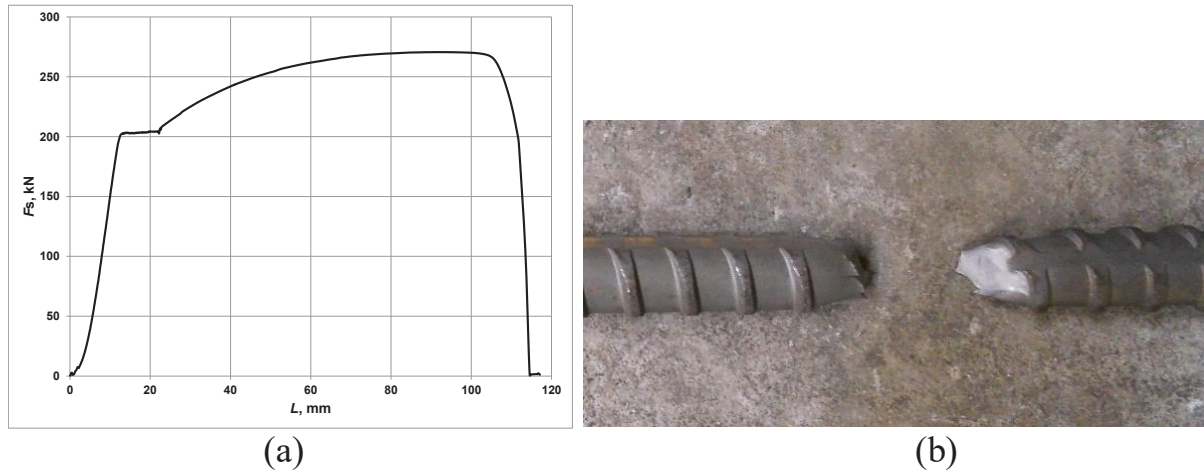
Figure 5: Bolt rod test under static tensile loading: (a) – loading course as a function of bolt rod elongation; (b) – ruptured rod after the test.
