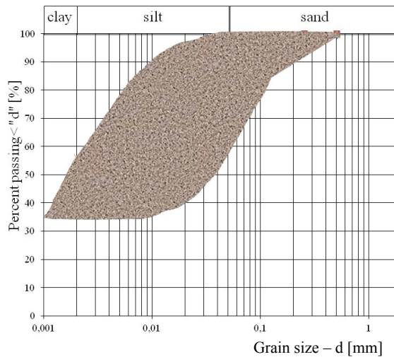
Fig. 4. Particle size distribution of Stegny clay
