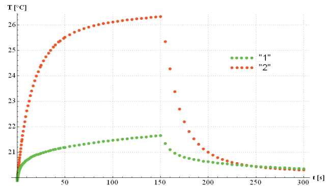
Fig. 7. Temperature curves for the medium with 25% polystyrene foam balls; “1” – sensor in the center of the inclusion, “2” – sensor at the longest distance from the inclusion
