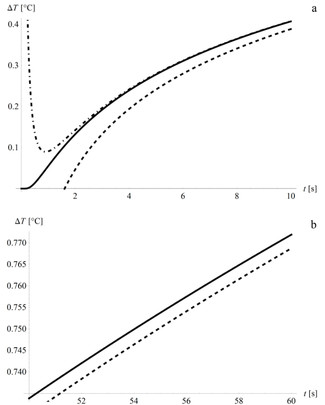
Fig. 3. The temperature increase \Delta T for two different time intervals.
