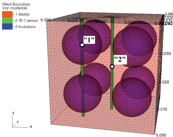
Fig. 5. Positions of the sensor considered in numerical simulations
