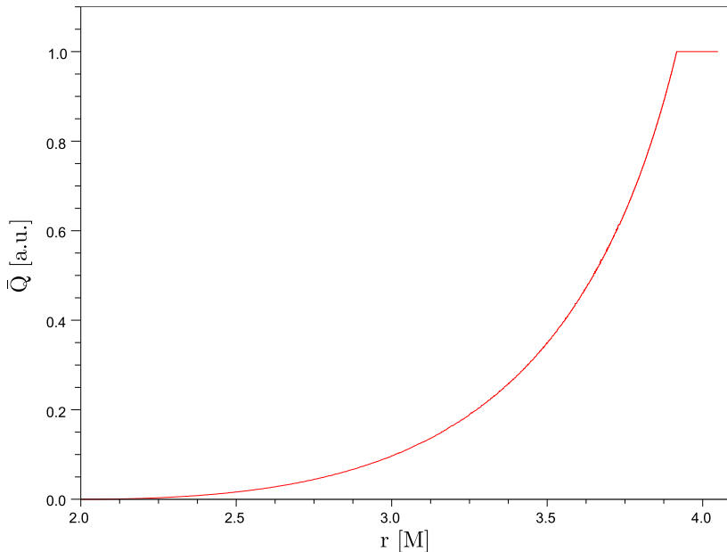
Figure 3.4. Average communication weight as a function of the radial coordinate r of the outer end of the rod during crossing the horizon.
